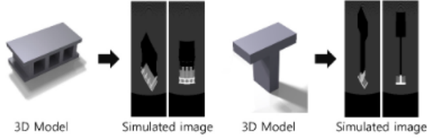
Figure 5: Ray tracing simulator using second method. (source: [25])
